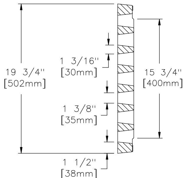
GRATE SECTION
