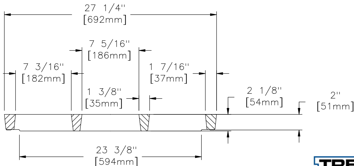
GRATE SECTION
